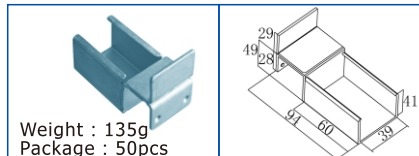
KJ-2044D(Zinc/Nickel/Chrome)
