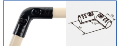
KJ-17
