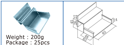
KJ-2085D(Zinc/Nickel/Chrome)
