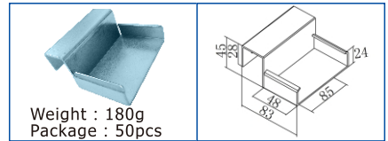
KJ-2085E(Zinc/Nickel/Chrome)
