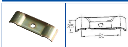
K-1000D(ZINC)
