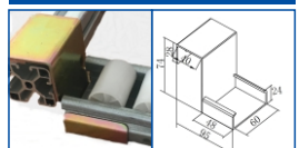
KJ-2060DW-40
