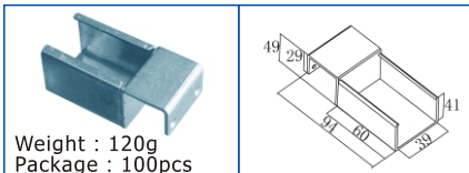
KJ-2044C(Zinc/Nickel/Chrome)
