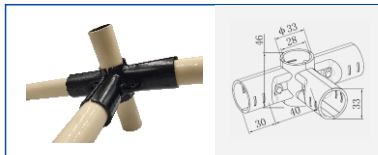
KJ-30-3
