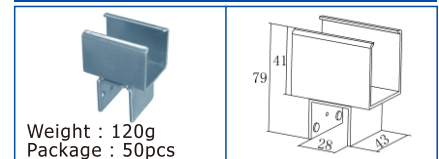
KJ-2044P(Zinc/Nickel/Chrome)
