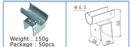
KJ-2044FF(Zinc/Nickel/Chrome)
