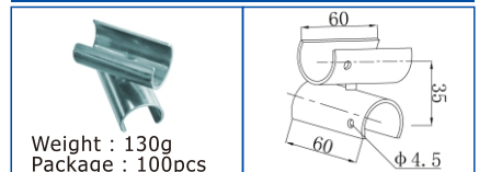
KJ-2044FF(Zinc/Nickel/Chrome)
