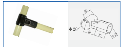
KJ-30-4
