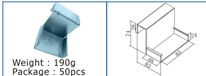
KJ-2085DW(Zinc/Nickel/Chrome)
