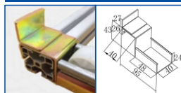
KJ-2044DW-40
