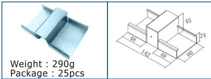
KJ-2085D(Zinc/Nickel/Chrome)
