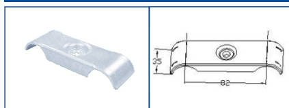
K-1003F
