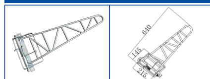
K-1005B
