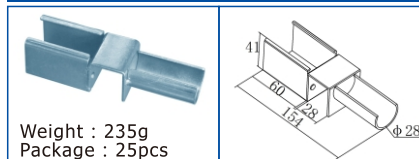
KJ-2044EF(Zinc/Nickel/Chrome)
