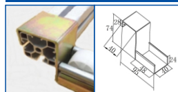
KJ-2060D-40
