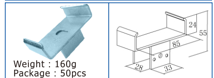
KJ-2085P(Zinc/Nickel/Chrome)
