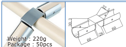
KJ-2044EC(Zinc/Nickel/Chrome)
