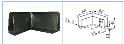
J-A3-10
