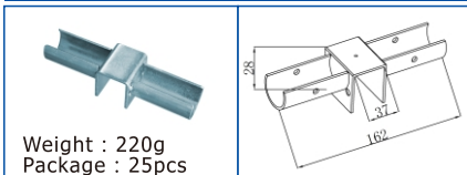
KJ-2044EH(Zinc/Nickel/Chrome)
