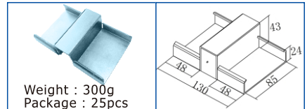
KJ-2085P(Zinc/Nickel/Chrome)
